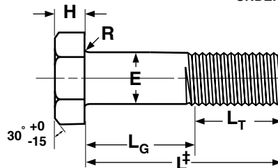
Cut Thread
