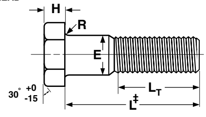
Rolled Thread
